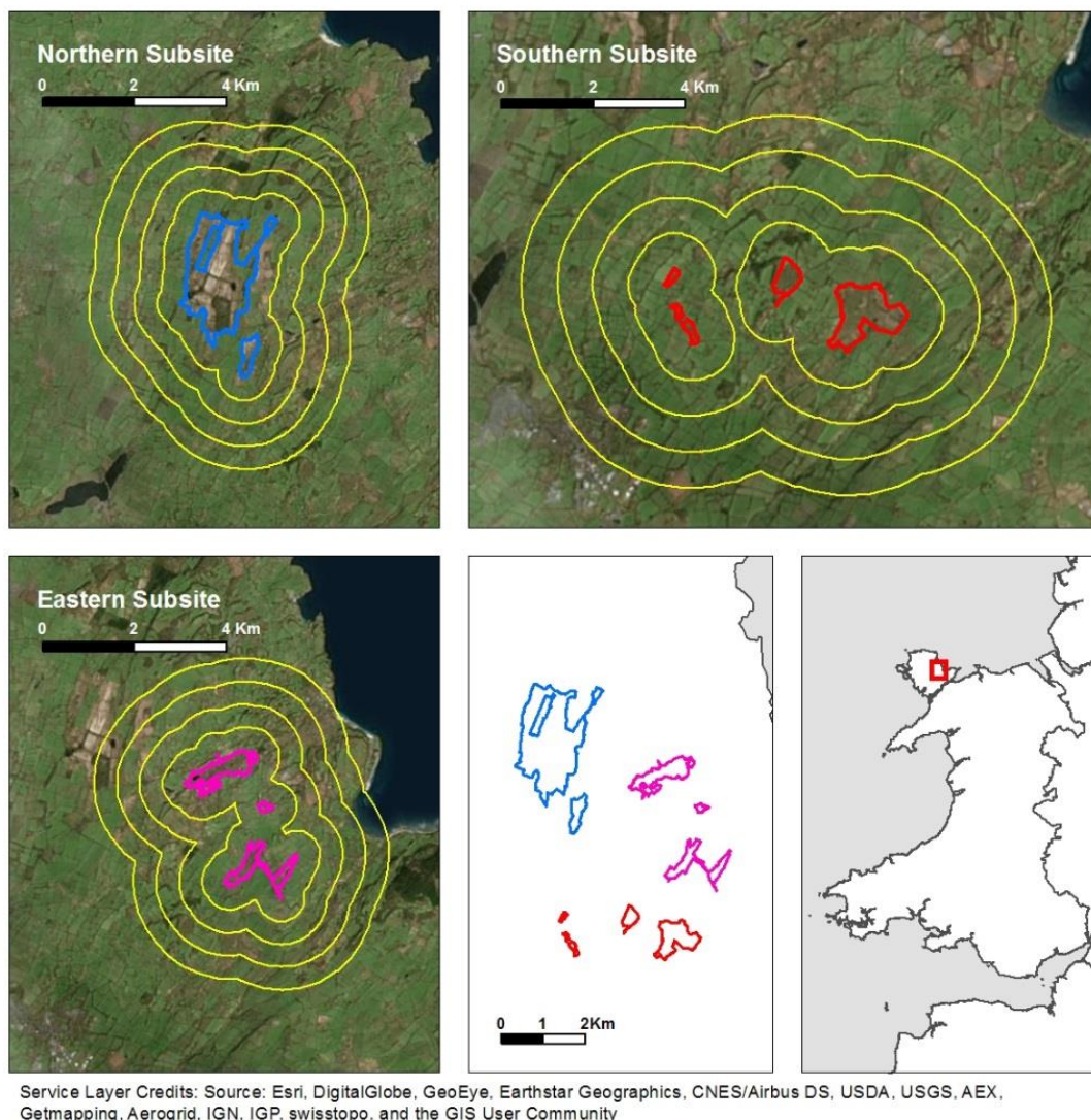
Figure 3-2 – Location of the sub-sites of Anglesey Fens SAC, with concentric 500 m buffer zones surrounding each sub site (up to 2 km) distance from the site boundaries.
