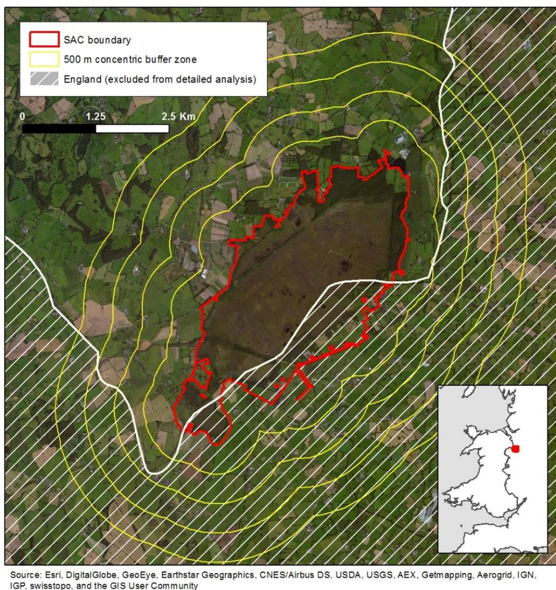
Figure 4-2 – Location of Fenn's, Whixall, Bettisfield, Wem and Cadney Mosses SAC, with concentric 500 m buffer zones surrounding the site (up to 2 km).
